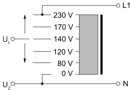
ATV connection diagram
